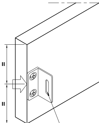
Fascia (vista retro) Band (rear view)
